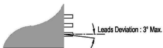
DETAIL A
