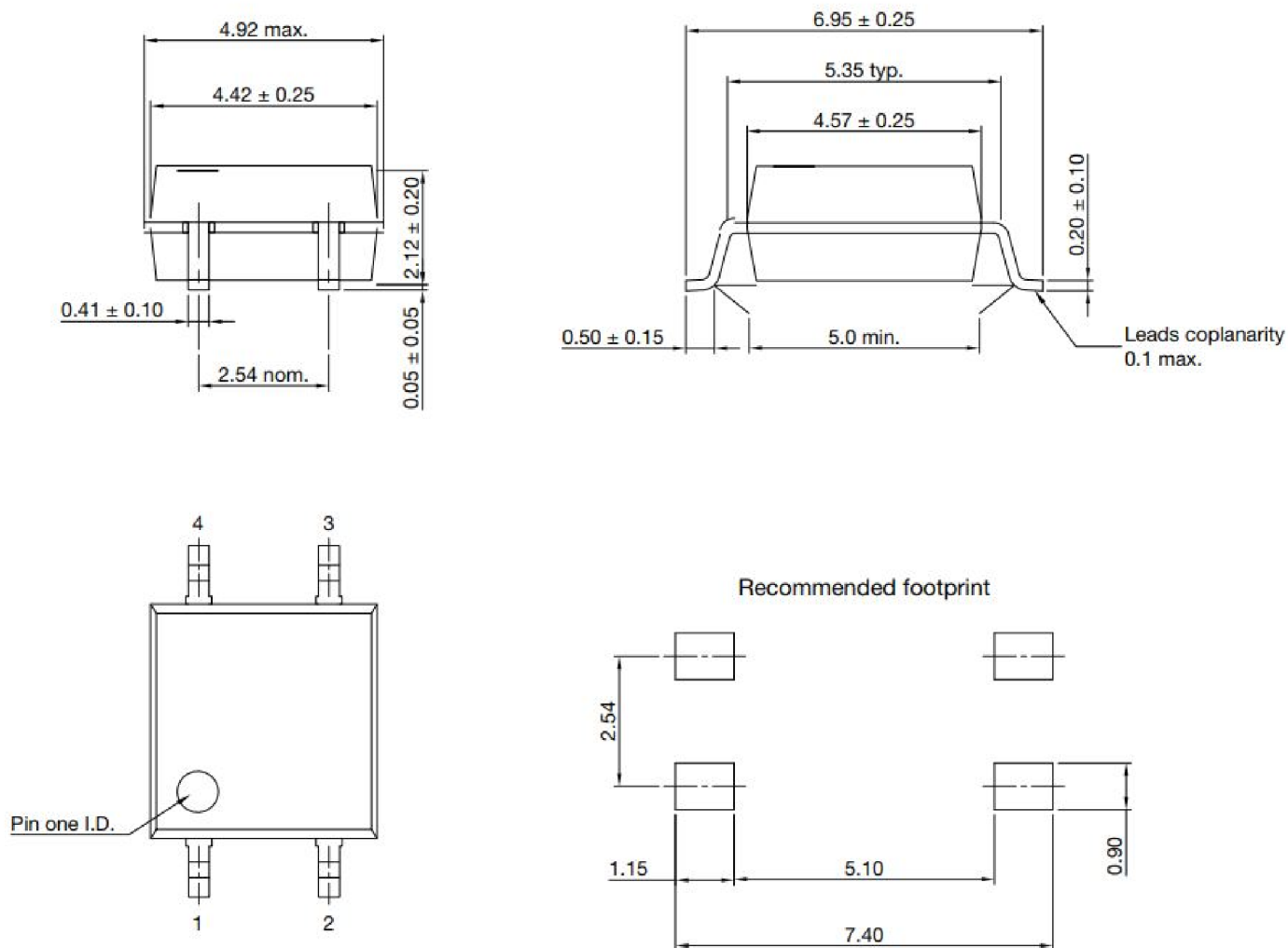
Fig. 11 - Package Drawings
