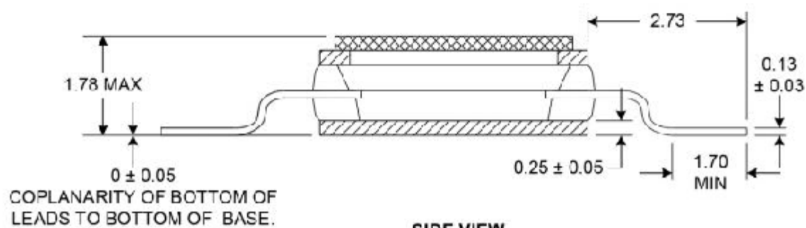
SIDE VIEW
