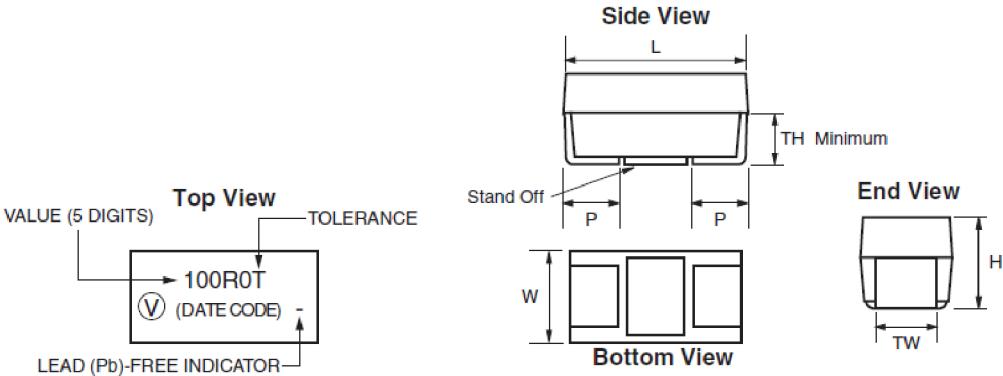
FIGURE 2 - DIMENSIONS in inches (millimeters)
