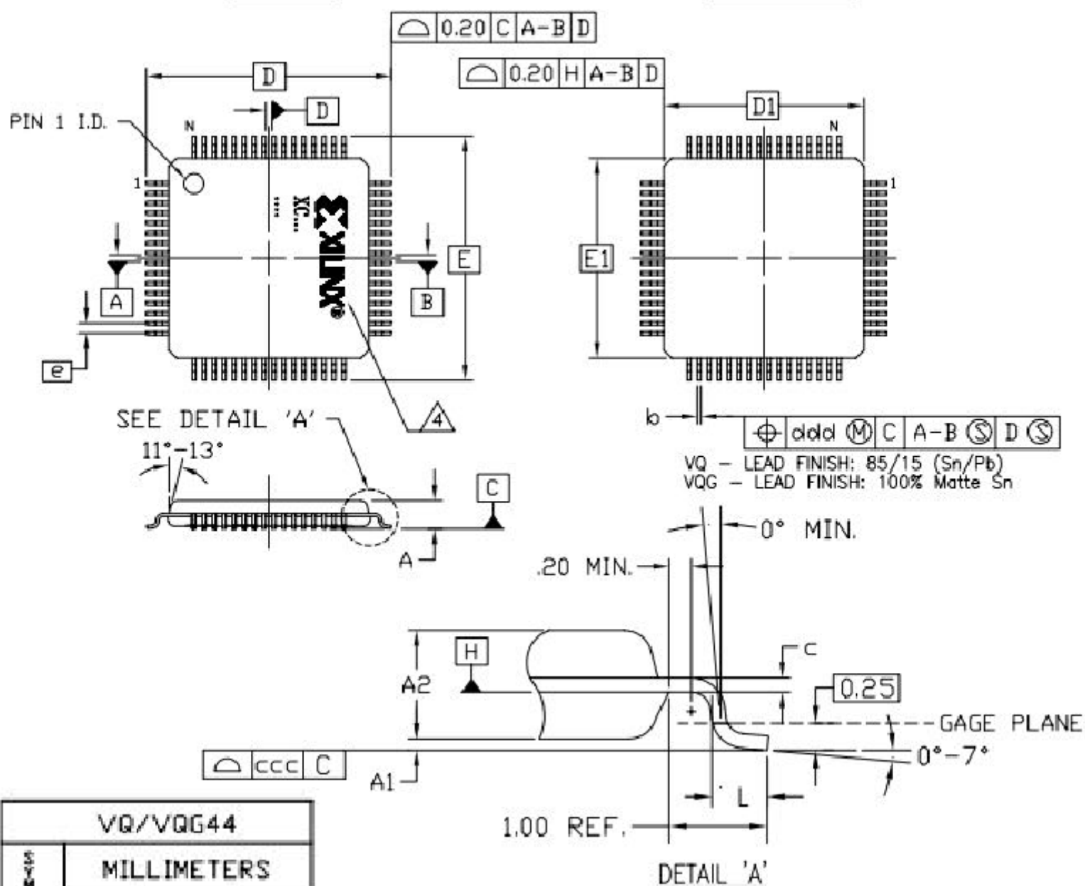
TOP VIEW
