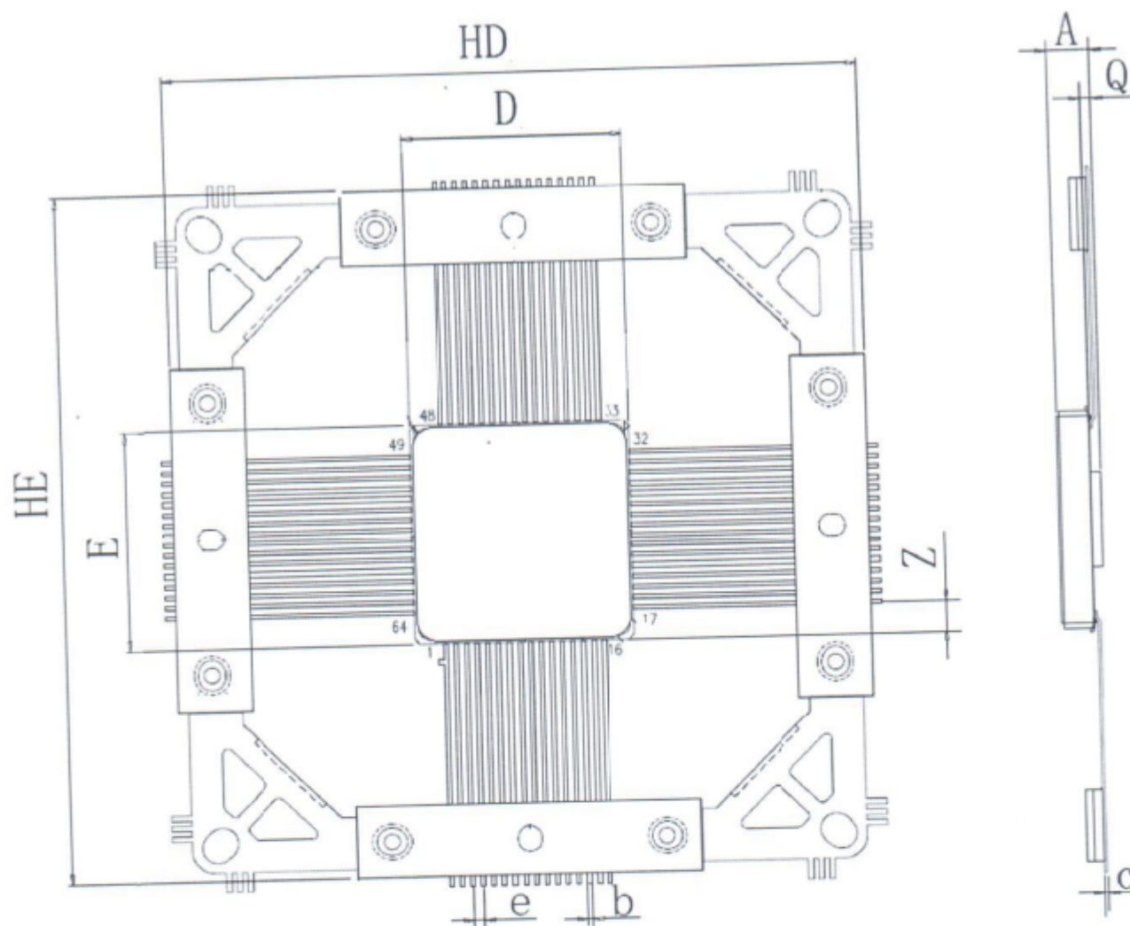
Figure 3.2 B9643RQC/B9643NQC Outline Dimensions
