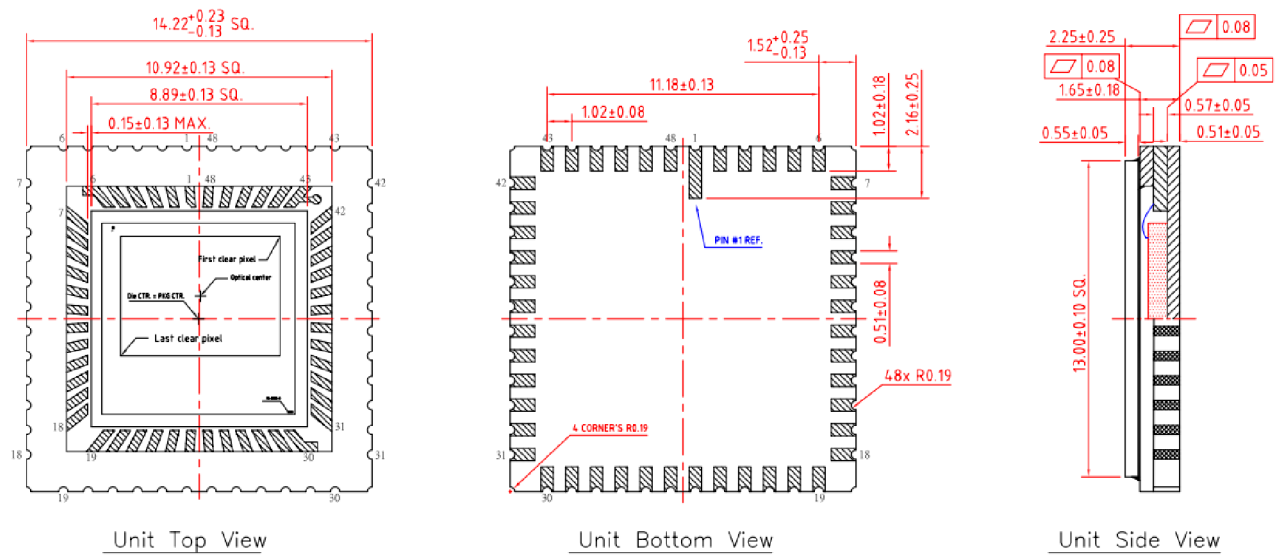
Figure 25: 48-Pin CLCC
