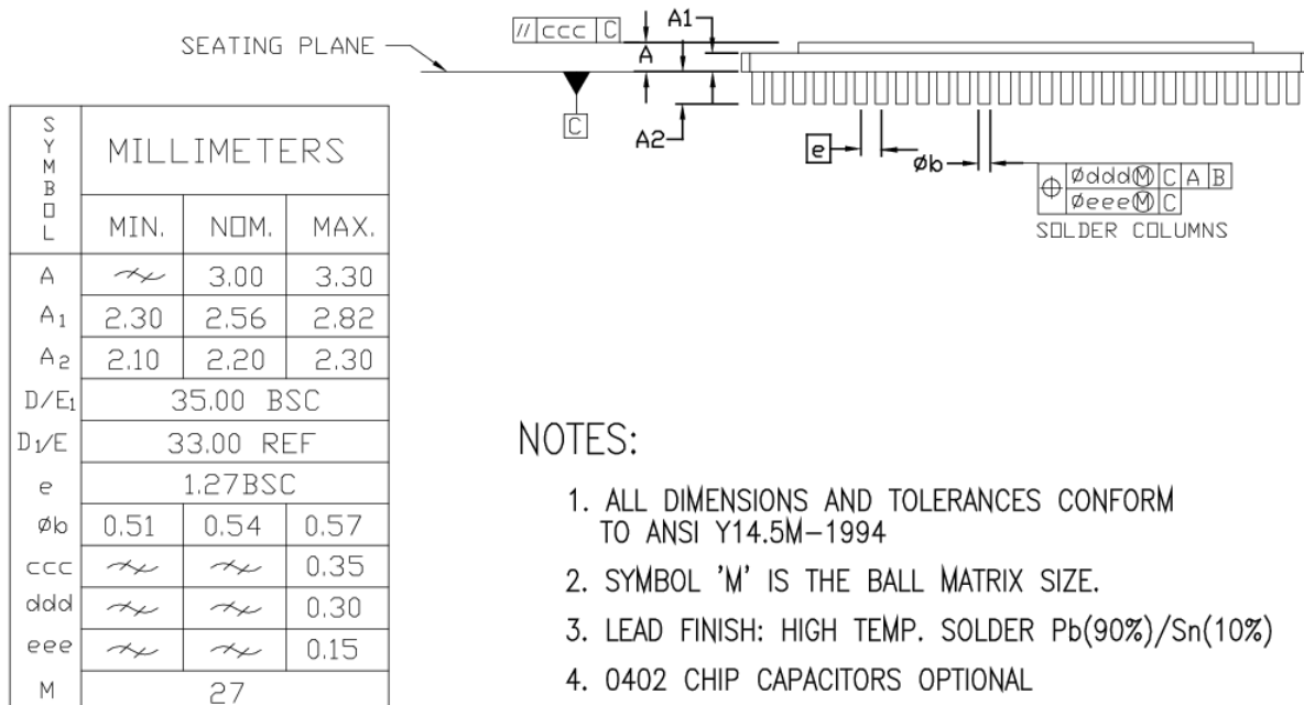
Figure 60: CG717 Ceramic CGA Package Specifications
