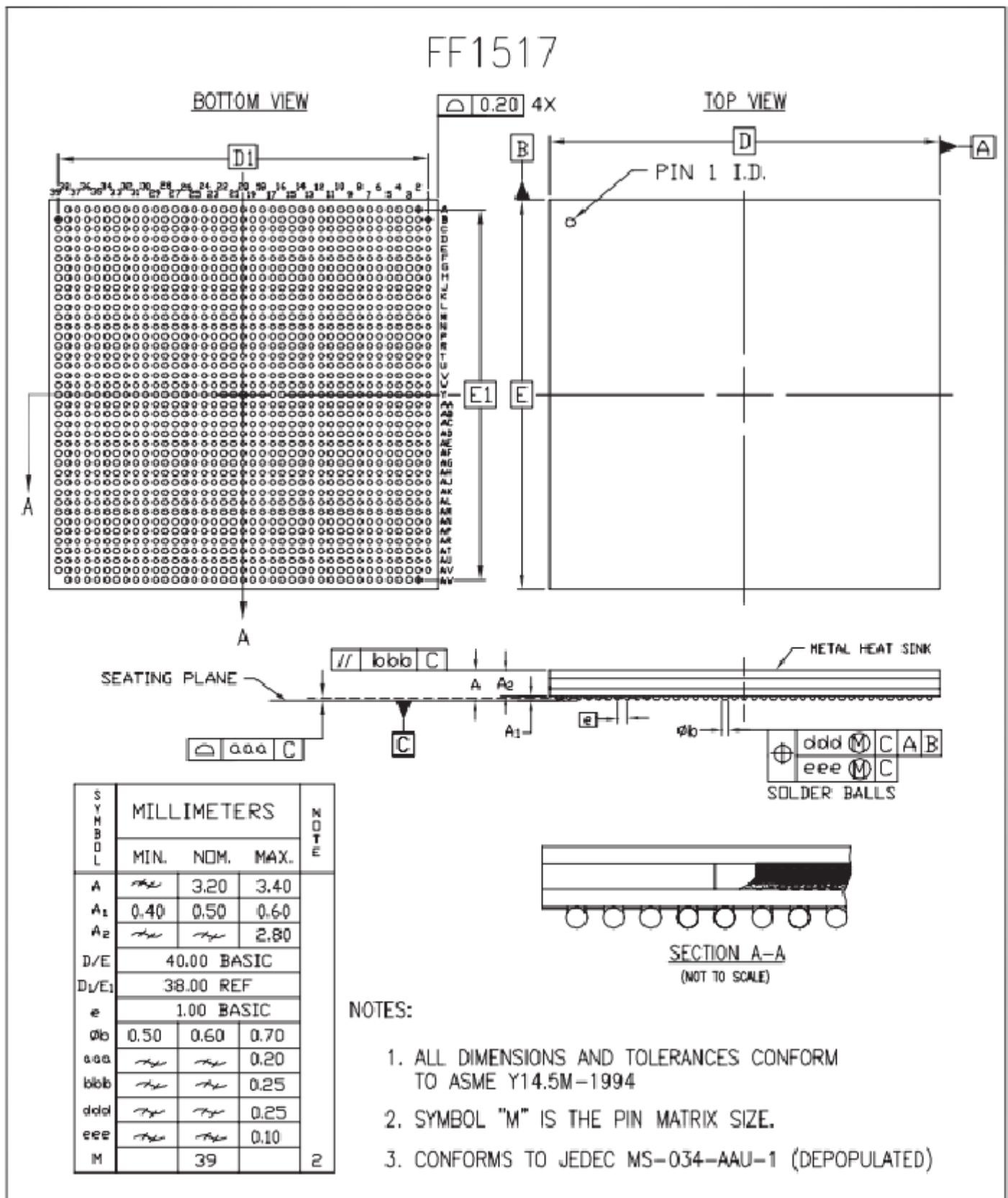
Figure 8: FF1517 Flip-Chip Fine-Pitch BGA Package Specifications
