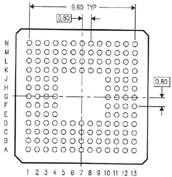
Bottom View
