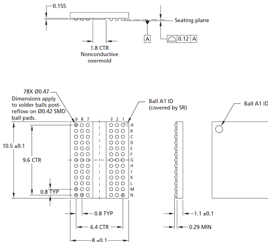
Figure 9: 78-Ball FBGA – x4, x8 (DA)
