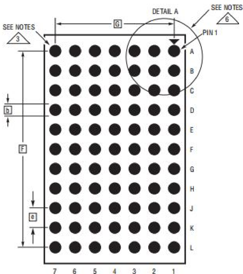
PACKAGE BOTTOM VIEW
