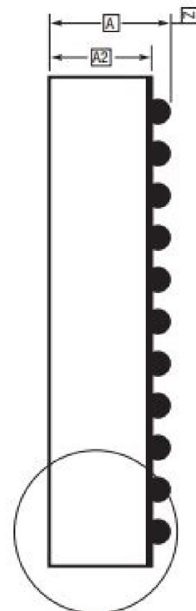
DETAIL B PACKAGE SIDE VIEW
