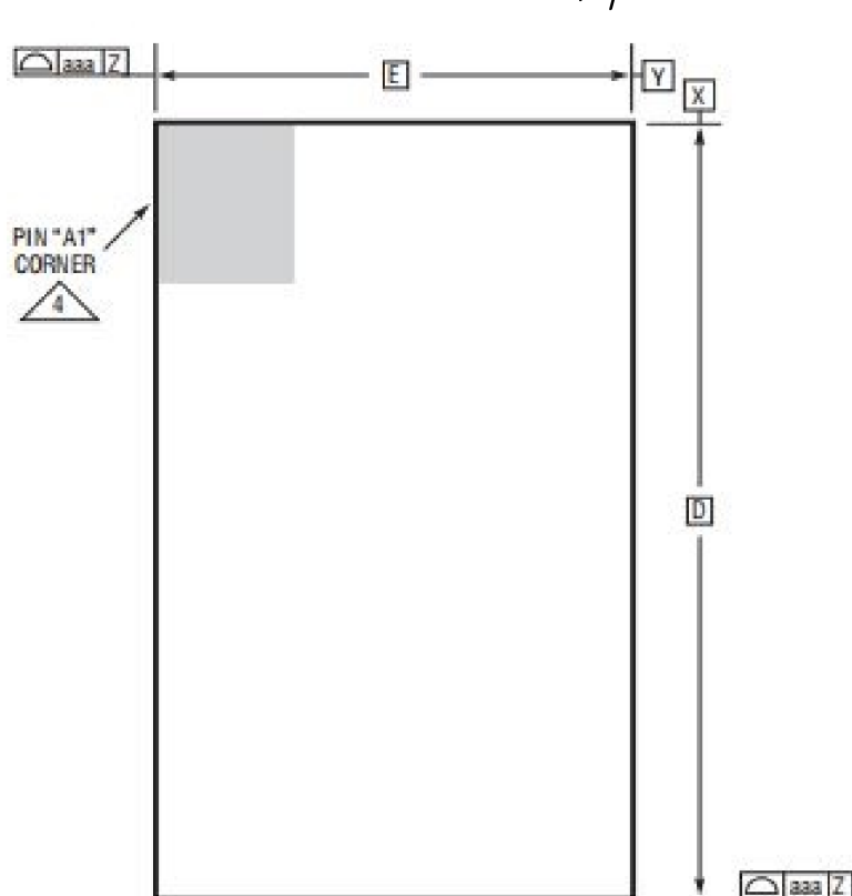
PACKAGE TOP VIEW
